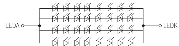
BACKLIGHT CIRCUIT DIAGRAM
